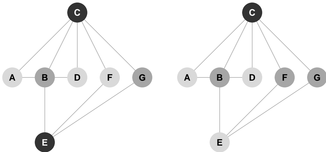
Figure 1: A requirement CIG with two different colourings.
