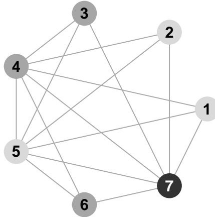
Figure 4: Estimability CIG of the unblocked MA fraction 7-2.1, coloured in terms of the successful mapping for Example 7 (this is of course no proper colouring for this CIG). The generating contrasts for the fraction are: factor 6 from the 3-factor interaction of factors 1, 2, and 3 and factor 7 from the 4-factor interaction of factors 1, 2, 4, and 5.
